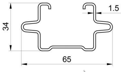
Standard-Haken
